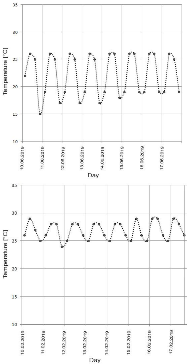
Figure 5: Temperature profile of the soil in Ankarafantsika at a depth of 20 cm during the dry (on top) and the rainy season (bottom).
